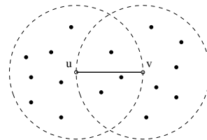
Fig. 1. The interference of link uv is the number of wireless nodes whose distance to node u or to node v is less than \|uv\| .
