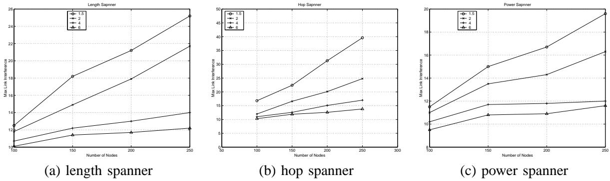
Fig. 5. The maximum interference of the optimum structures with different length spanning ratio requirement (a), hop spanning ratio requirement (b), and power spanning ratio requirement (c).
