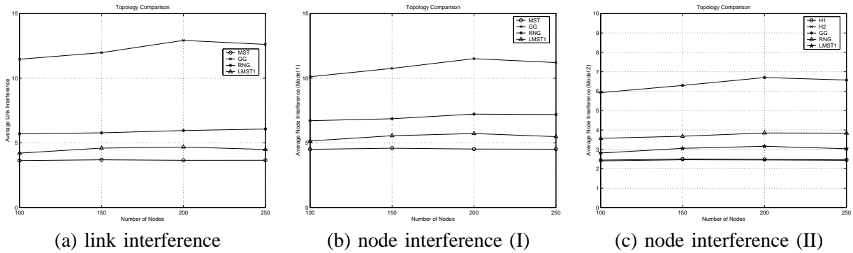
Fig. 7. Comparison of various topologies in terms of the average link interference (a), the average node interference defined by the first model (b), and the average node interference defined by the second model (c).
