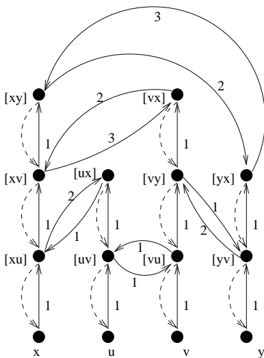
Fig. 3. The transformed graph.
