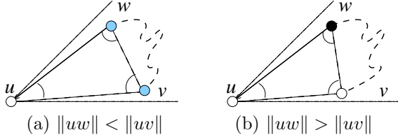
Fig. 2. Two cases when uv is removed while processing u .
