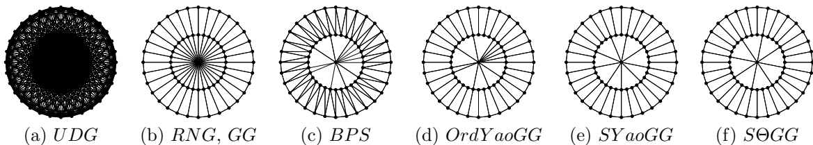
Fig. 1. Several planar power spanners on the UDG shown in (a). Here k = 9 during constructing SYaoGG and S\Theta GG .
