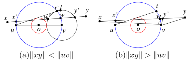
Fig. 8. Two hypothetical cases that an edge uv is not isolated
