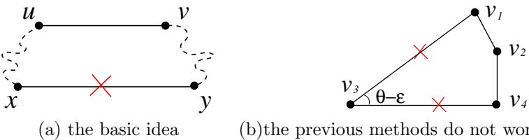
Fig. 3. Illustration of the method to build low-weighted graph
