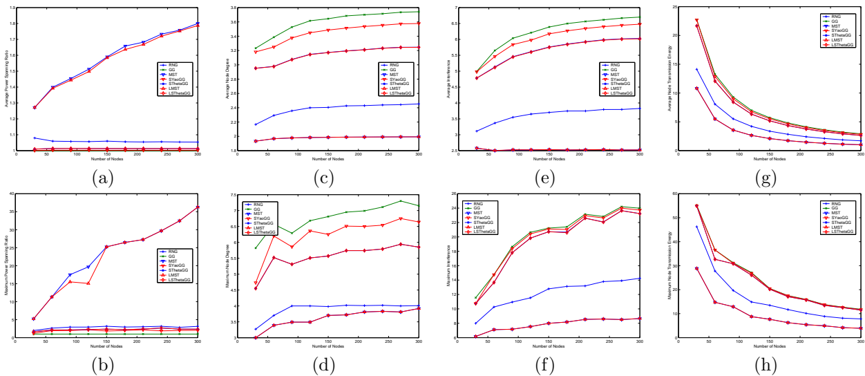
Fig. 7. The average and maximum performances of various structures. (a)(b) average and maximum power spanning ratio; (c)(d) average and maximum logical degree; (e)(f) average and maximum physical degree; (g)(h) average and maximum node power
