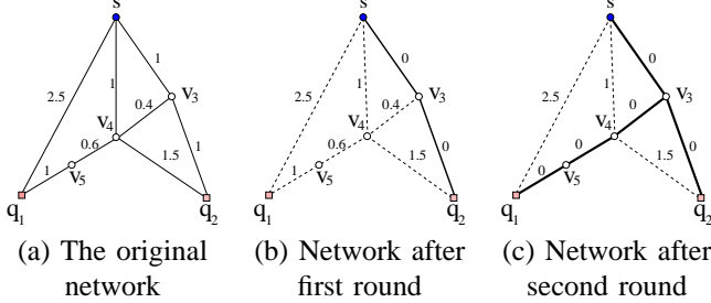
Fig. 1. Illustration of Algorithm (3). Here, s is the source node.
