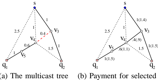
Fig. 2. Payment calculation based on LST found by Algorithm (3).
