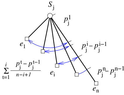
Fig. 6. Share the payment to service providers among receivers fairly.
