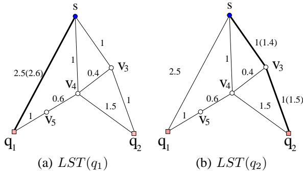
Fig. 3. LST(q_1) and LST(q_2) and their corresponding payment(3).
