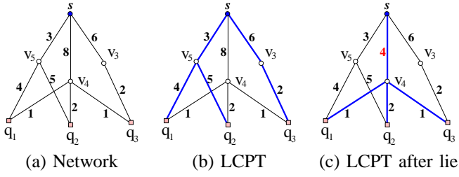
Fig. 4. VCG mechanism is not truthful for LCPT
