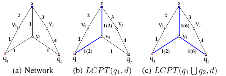
Fig. 5. ELSD charging scheme does not work for LCPT
