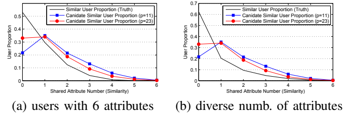
Fig. 5. Candidate user proportion with different similarity and prime number.
