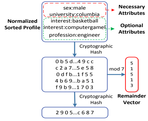
Fig. 2. The procedure to generate the profile key and remainder vector with a sample user profile.
