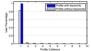
Fig. 4. Profile uniqueness and collisions of users.
