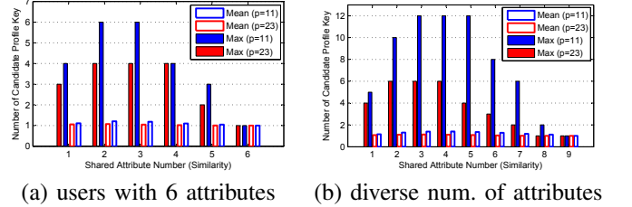
Fig. 6. Size of candidate profile key set with different similarities.
