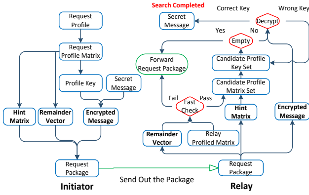
Fig. 1. The procedure to create a request package by the initiator and handle a request package by some forwarder.
